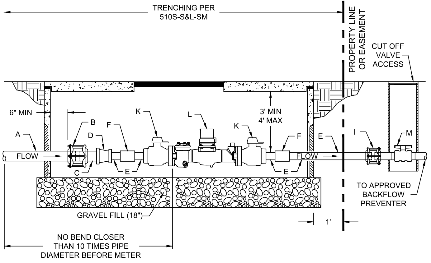
PROFILE VIEW
