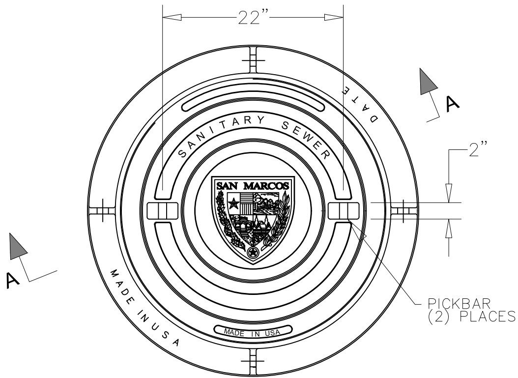
FRAME AND LID PLAN VIEW
