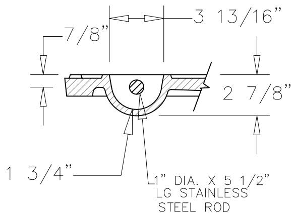
PICKBAR DETAIL
