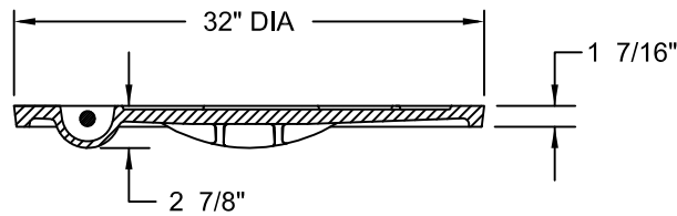
COVER SECTION
