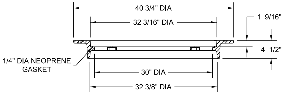
FRAME SECTION
