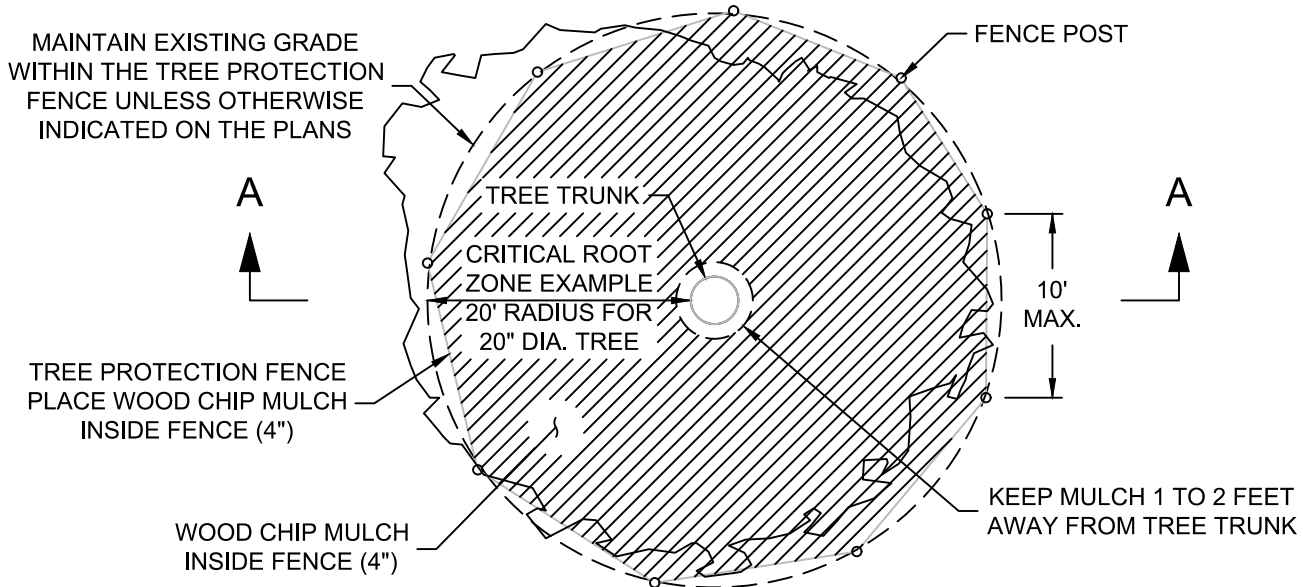
PLAN VIEW
