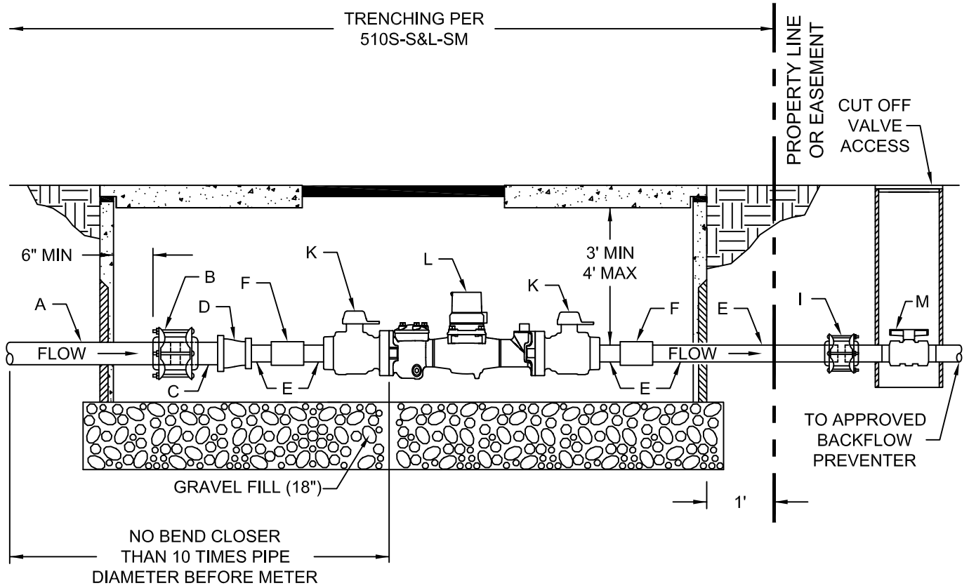
PROFILE VIEW
