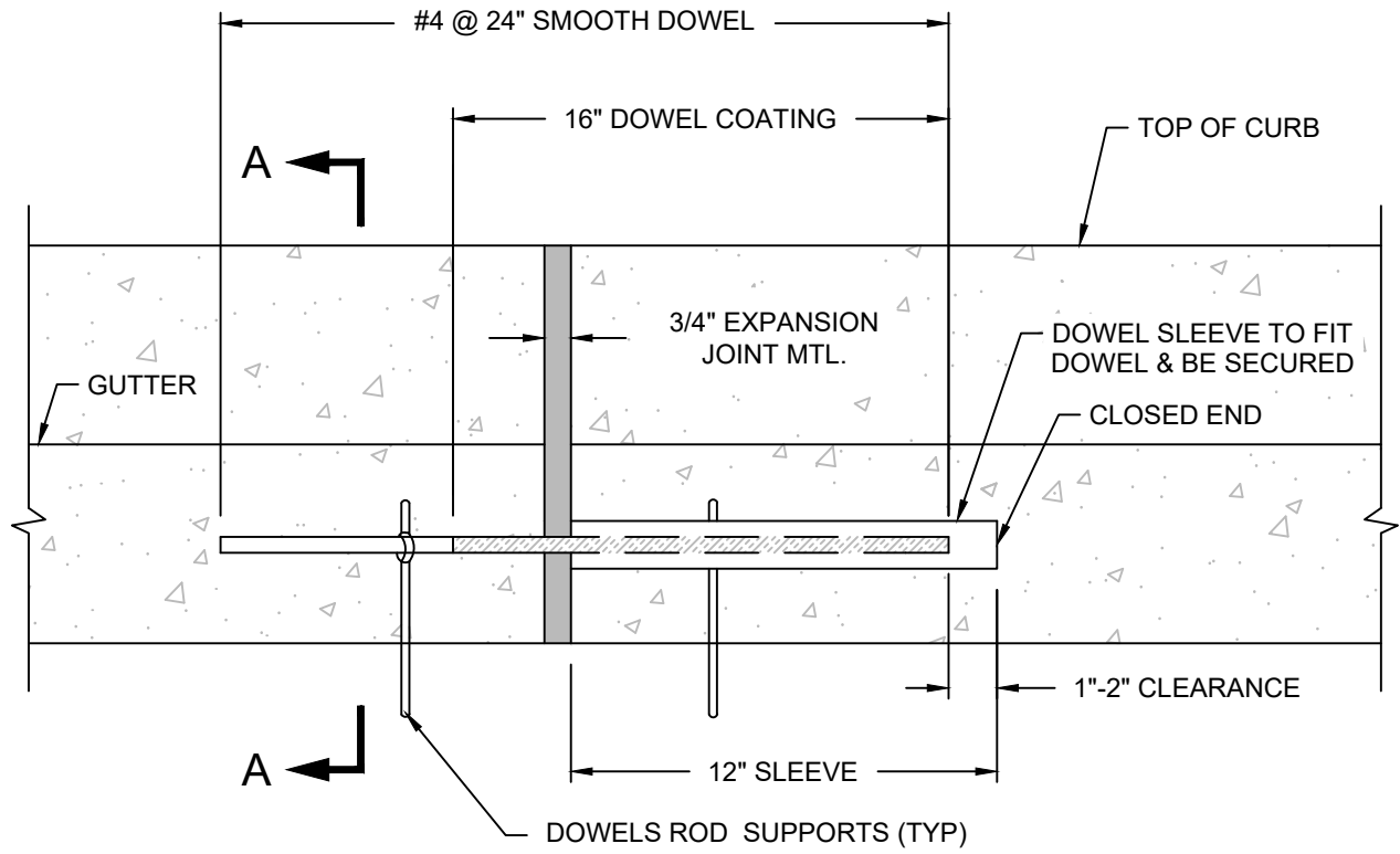
CURB EXPANSION JOINT DOWEL DETAIL
